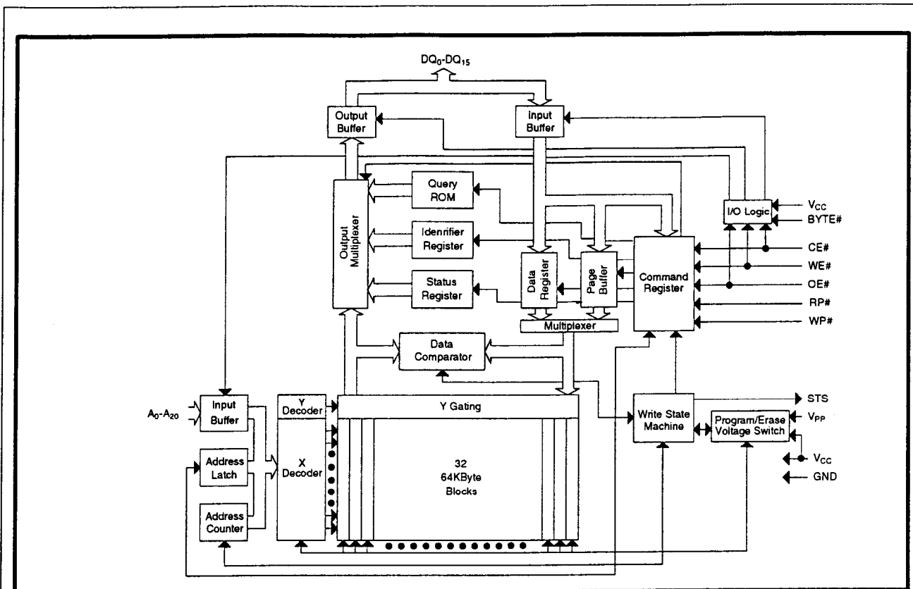
Figure 1. Block Diagram
