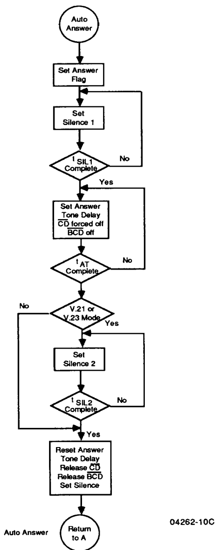
Figure 8. Autoanswer State Diagram
