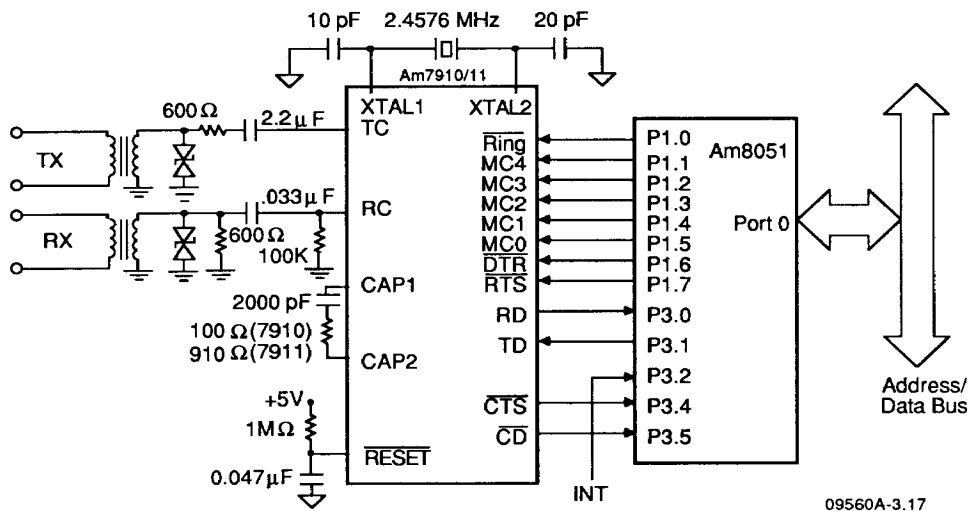
Figure 23. 1200 bps Four-Wire Full-Duplex Circuit
