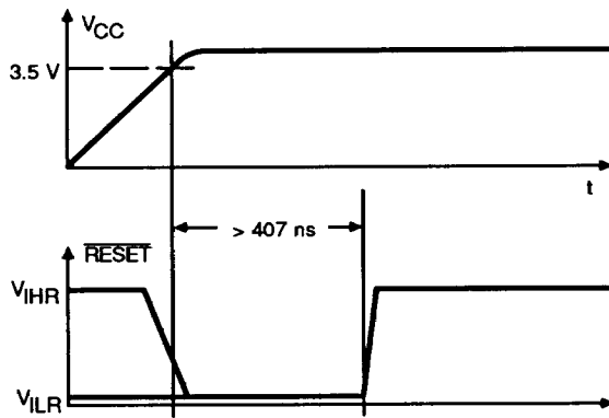
Figure 17. Reset Timing Diagrams
