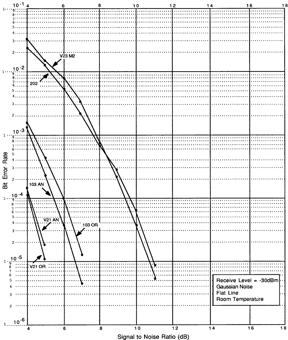
Figure 20. Am7910/11 Nominal Bit Error Rate
