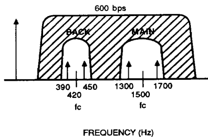
Figure 4. Full-Duplex Channel Assignments
