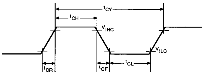
Figure 15. External Clock
