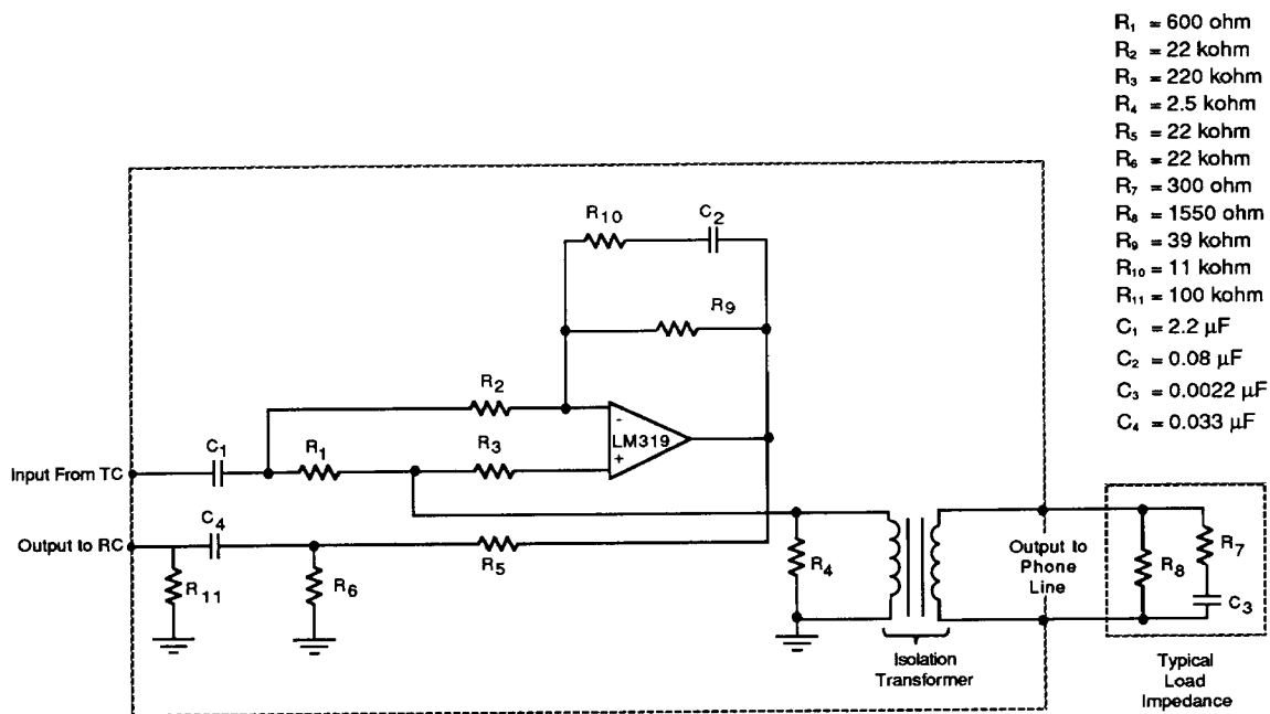
Figure 23. 1200 bps Four-Wire Full-Duplex Circuit
