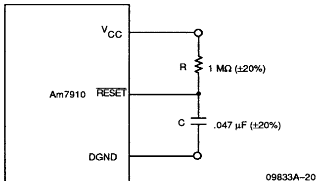
Figure 16. Automatic Reset
