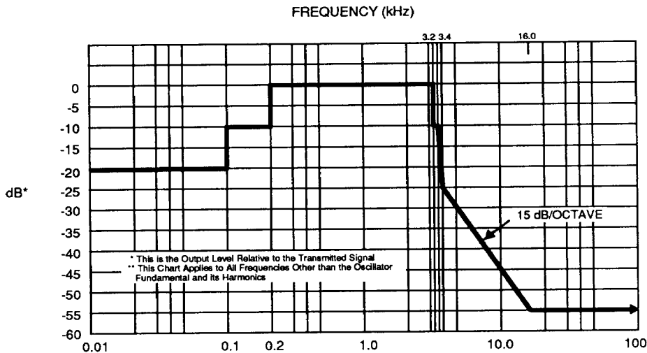
Figure 21. Out-of-Band Transmitter Energy
