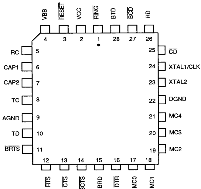
28-Pin PLCC
