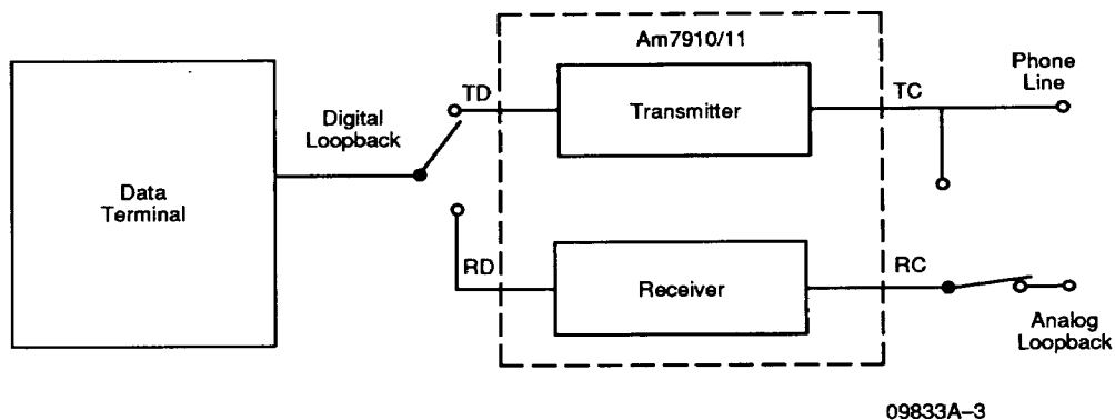
Figure 1. Analog Loopback
