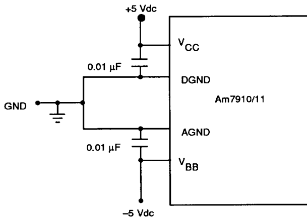
Figure 19. Power-Supply Connections
