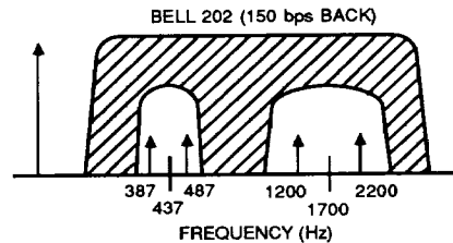
Figure 5. Half-Duplex Channel Assignments
