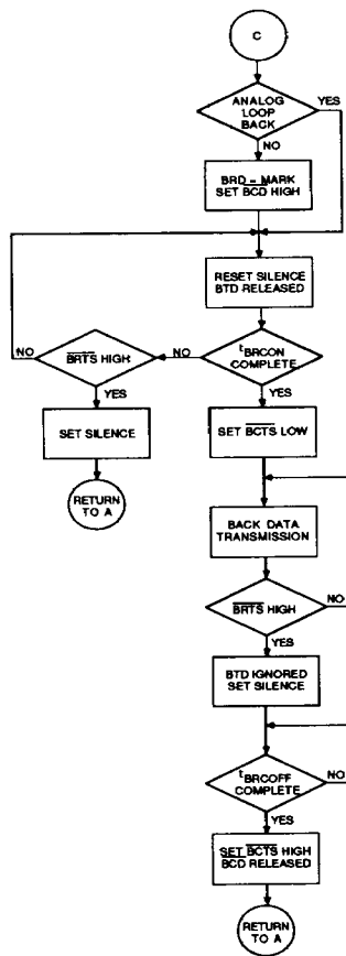
Figure 7. Transmit Back Channel State Diagram
