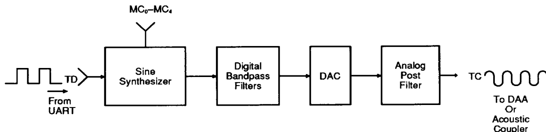
Figure 2. Transmitter Block Diagram
