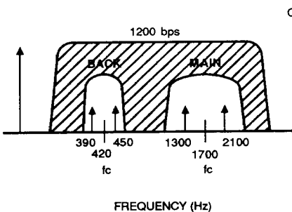
Figure 4. Full-Duplex Channel Assignments
