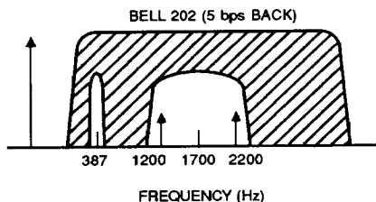
Figure 5. Half-Duplex Channel Assignments
