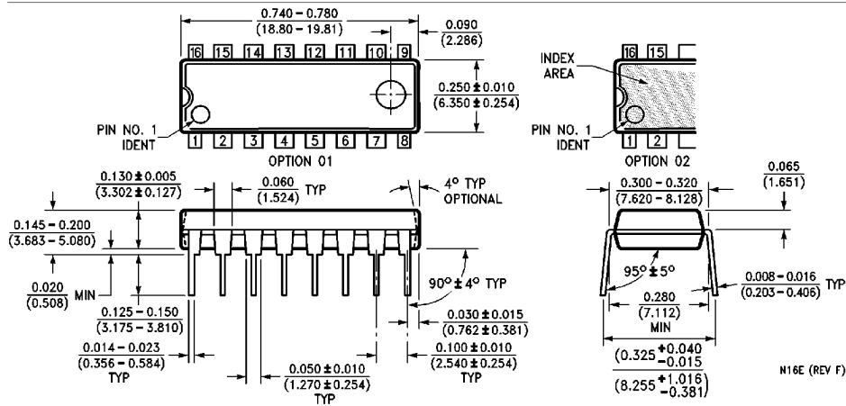
16-Lead Molded Dual-In-Line Package (N) Order Number DM74LS193N NS Package Number N16E
