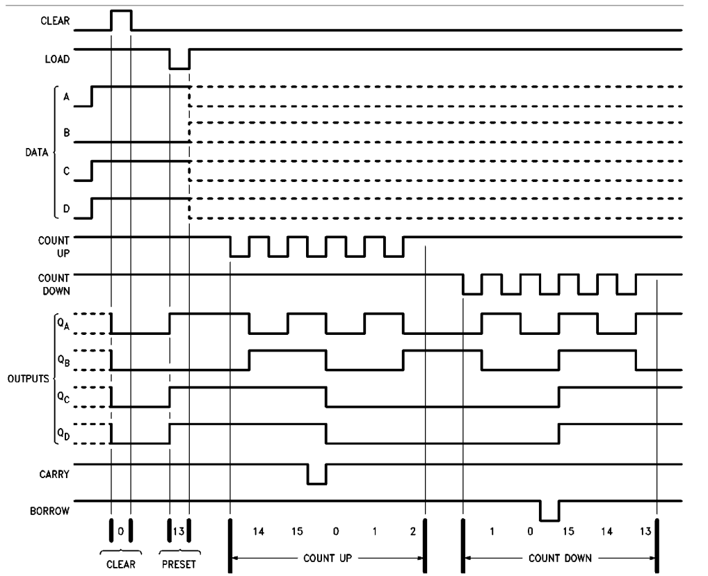
Typical Clear, Load, and Count Sequences
