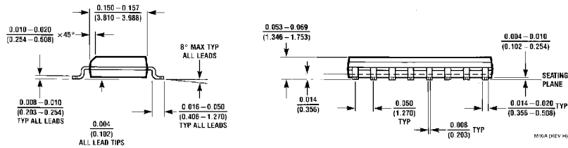
16-Lead Small Outline Molded Package (M) Order Number DM74LS193M NS Package Number M16A
