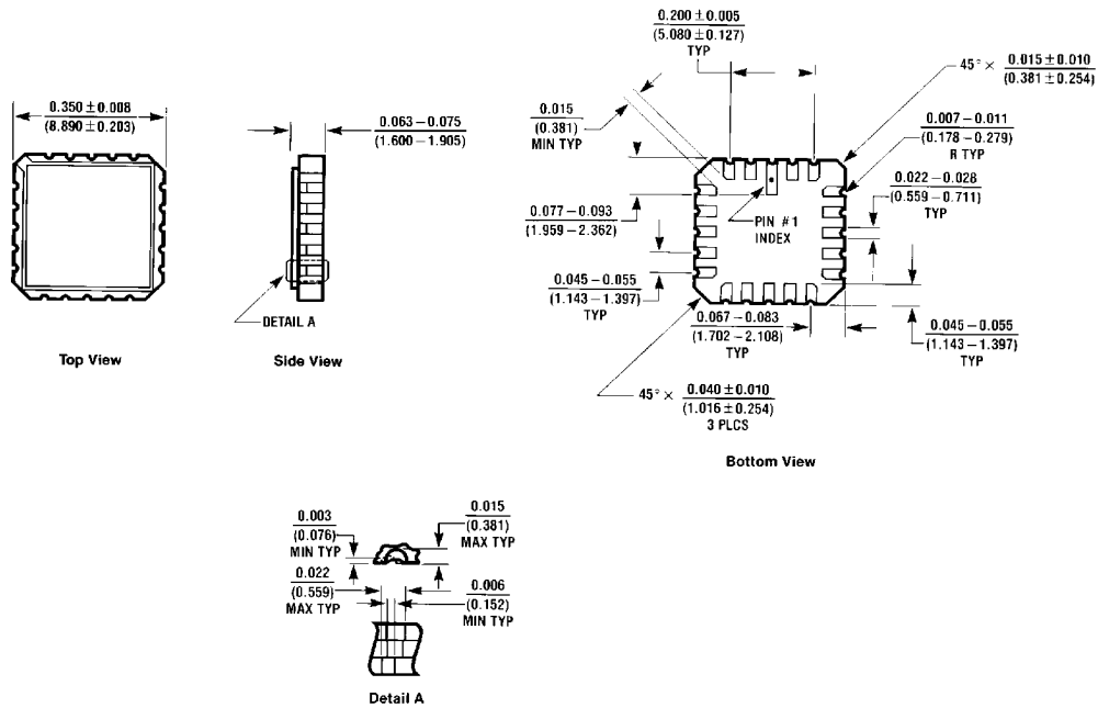
Ceramic Leadless Chip Carrier Package (E) Order Number 54LS193LMQB NS Package Number E20A
