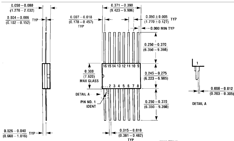
16-Lead Ceramic Flat Package (W) Order Number 54LS193FMQB or DM54LS193W NS Package Number W16A
