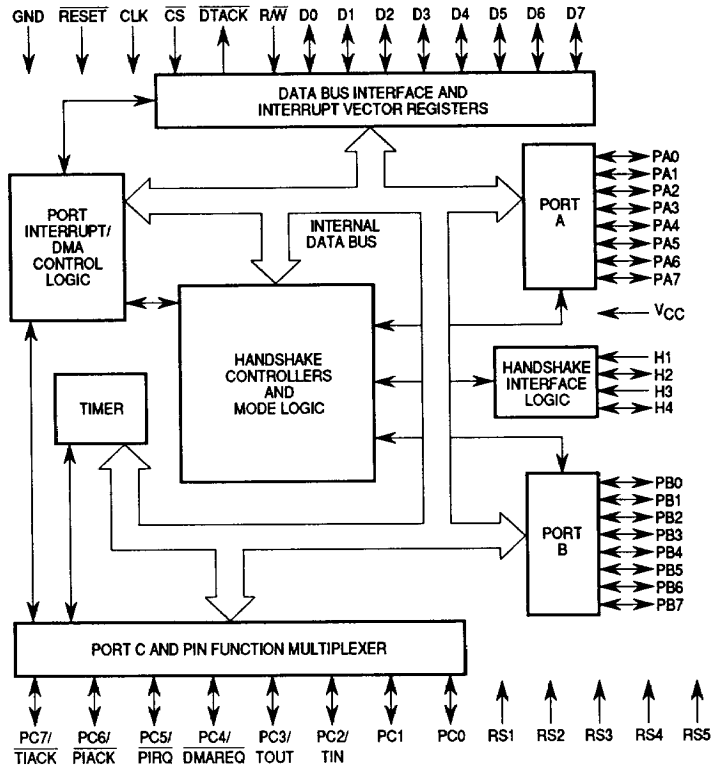
Figure 1. Block Diagram
