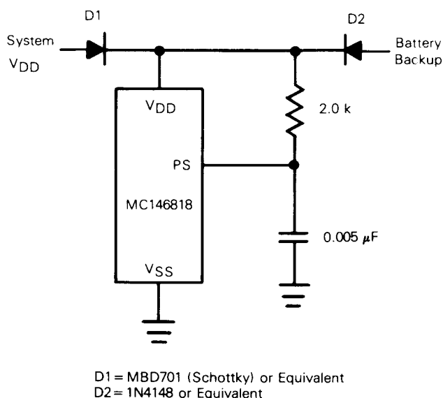
FIGURE 14 — TYPICAL POWERUP DELAY CIRCUIT FOR POWER SENSE
