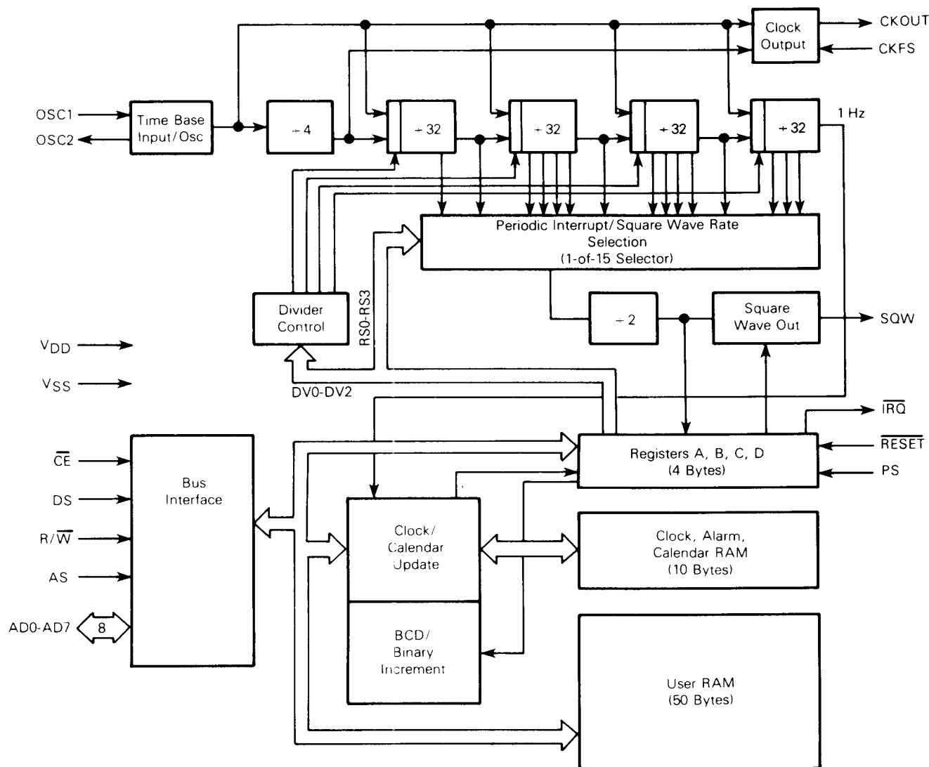
FIGURE 1 — BLOCK DIAGRAM
