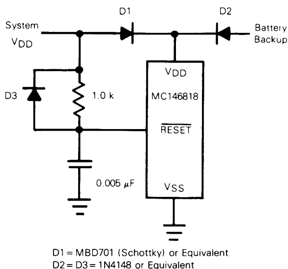
FIGURE 13 — TYPICAL POWERUP DELAY CIRCUIT FOR RESET
