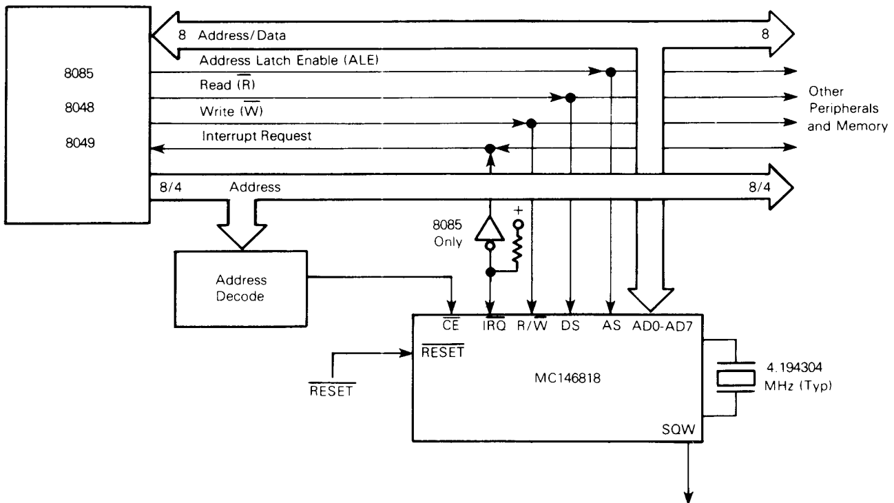
FIGURE 18 — MC146818 INTERFACED WITH COMPETITOR COMPATIBLE MULTIPLEXED BUS MICROPROCESSORS
