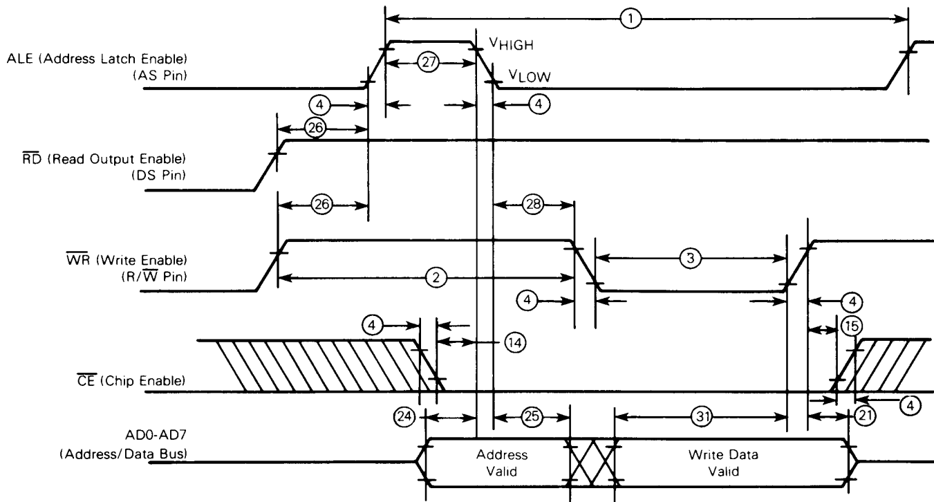
FIGURE 4 — BUS WRITE TIMING COMPETITOR MULTIPLEXED BUS
