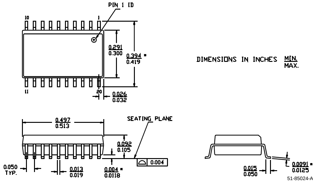
20-Lead (300-Mil) Molded SOIC S5
