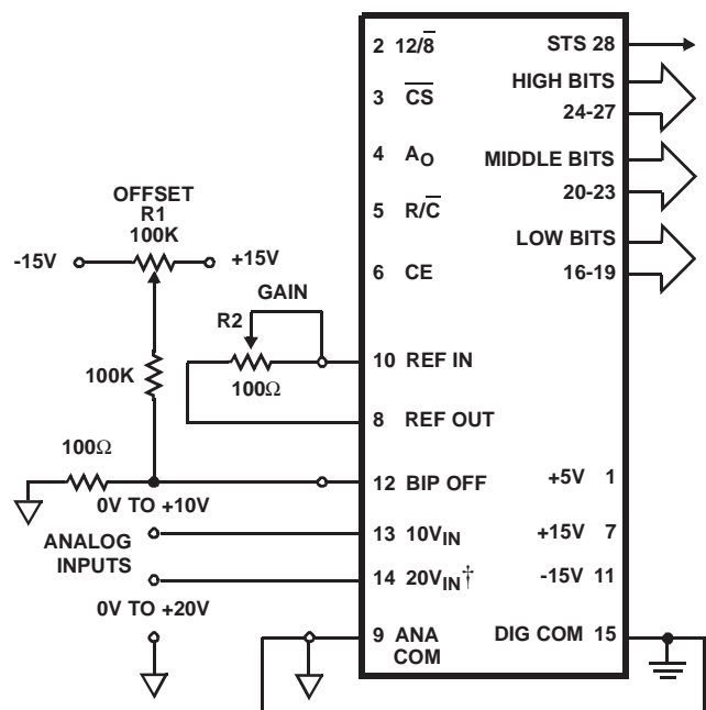
FIGURE 1. UNIPOLAR CONNECTIONS
