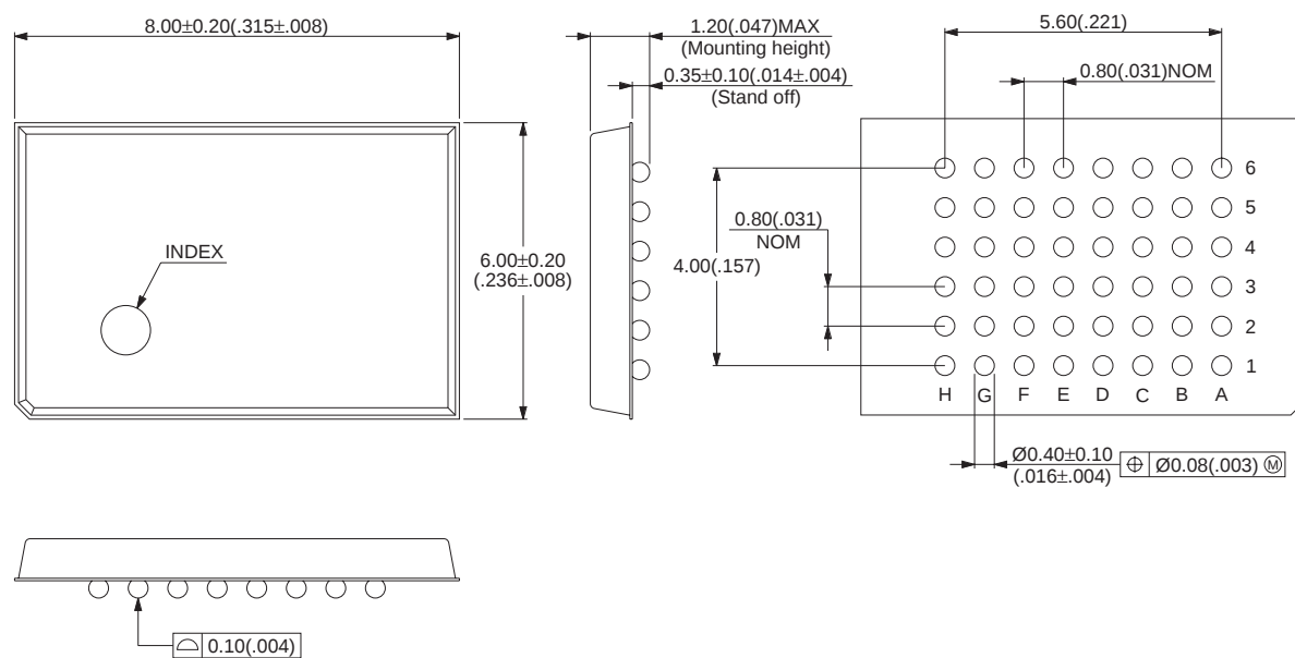
48-pin plastic FBGA (BGA-48P-M01)
