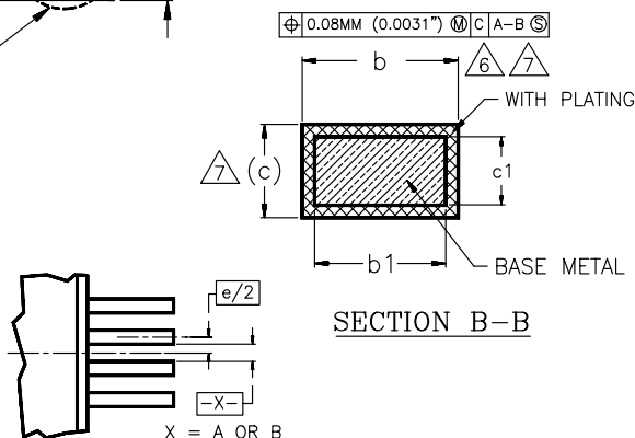
DETAIL B
