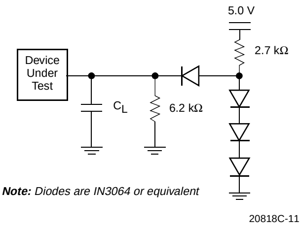
Figure 8. Test Setup
