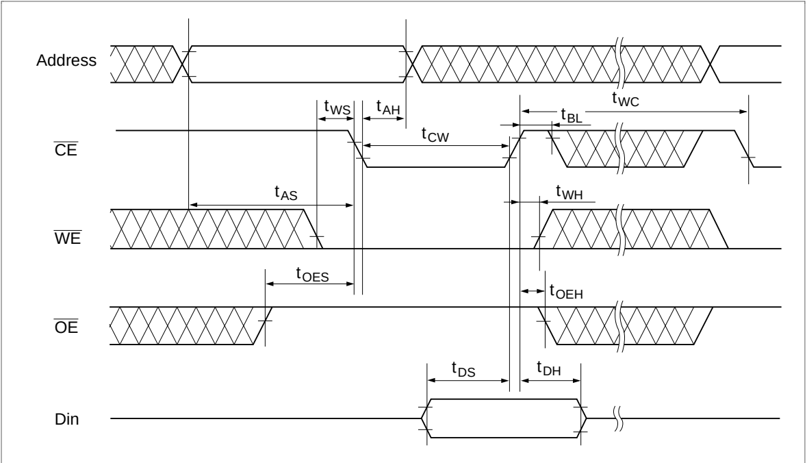
Page Write Timing Waveform (1) ( \overline{\text{WE}} Controlled)
