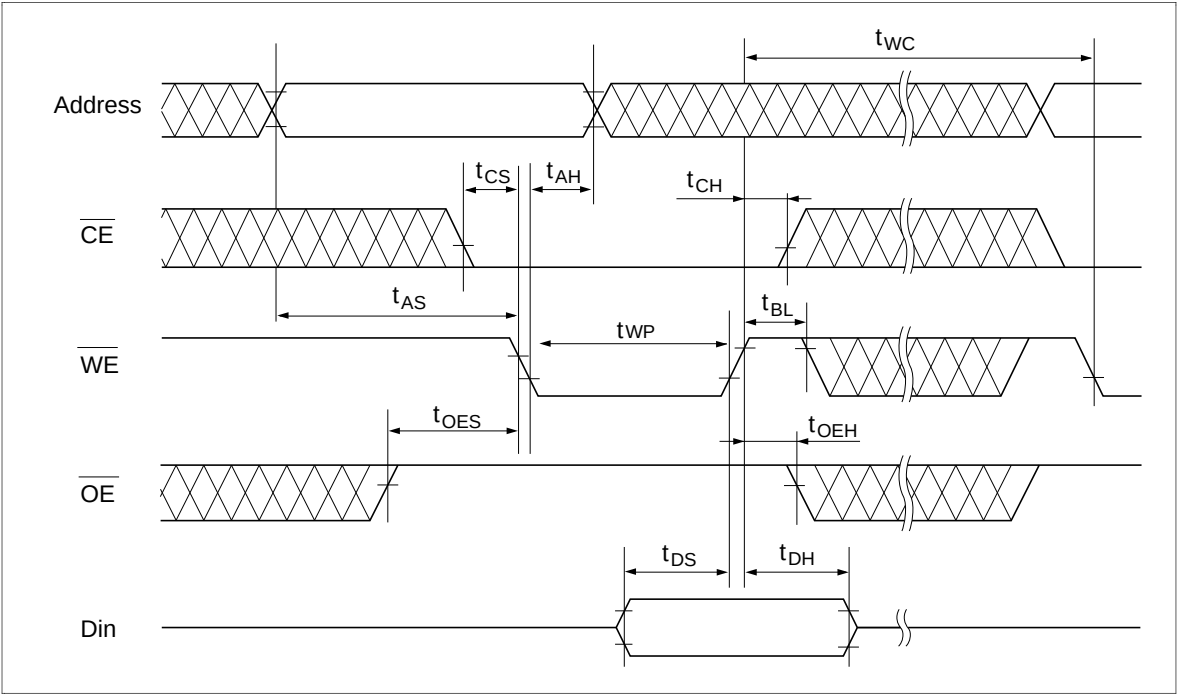
Byte Write Timing Waveform ( \overline{\text{CE}} Controlled)
