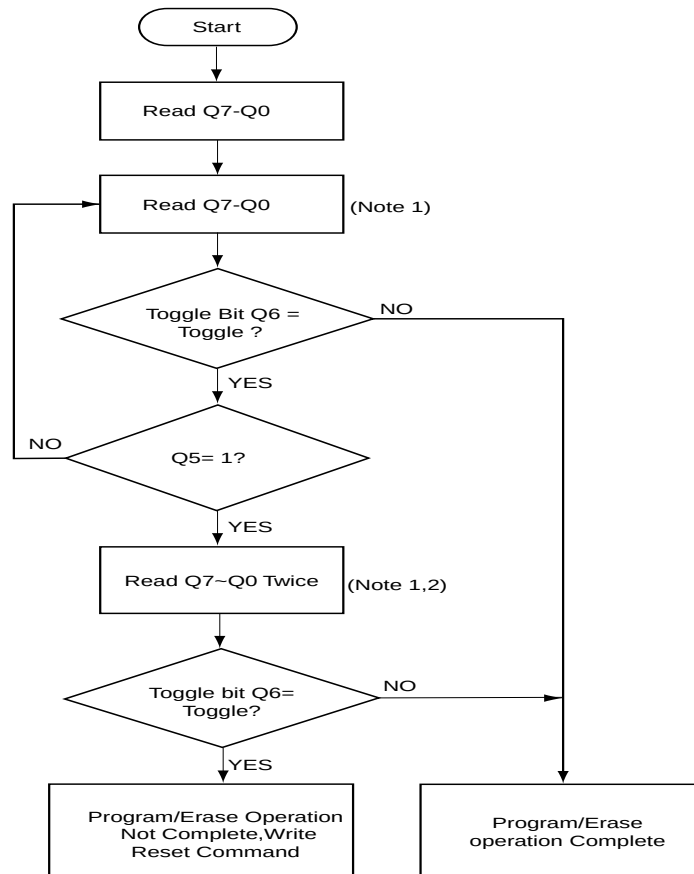
Figure 19. TOGGLE BIT ALGORITHM
