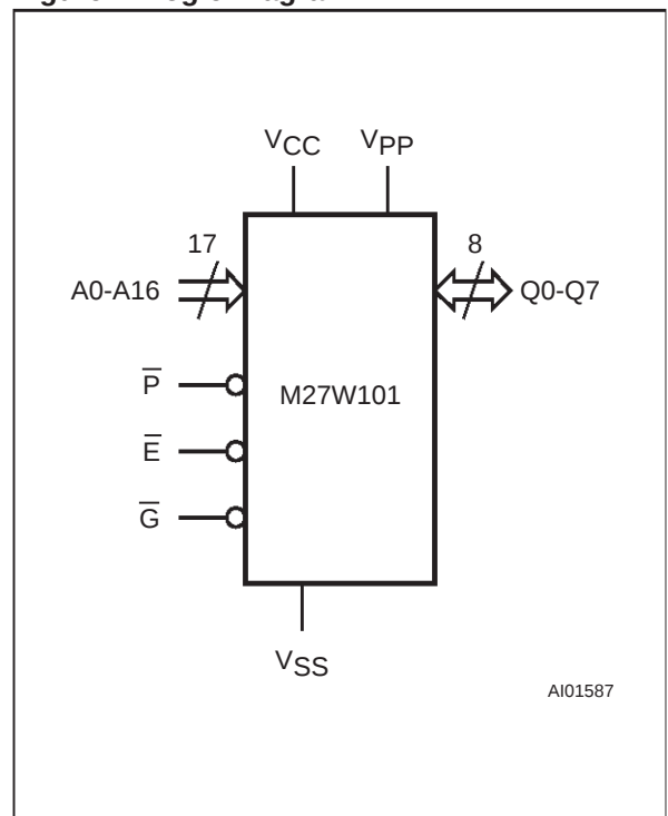
Figure 1. Logic Diagram
