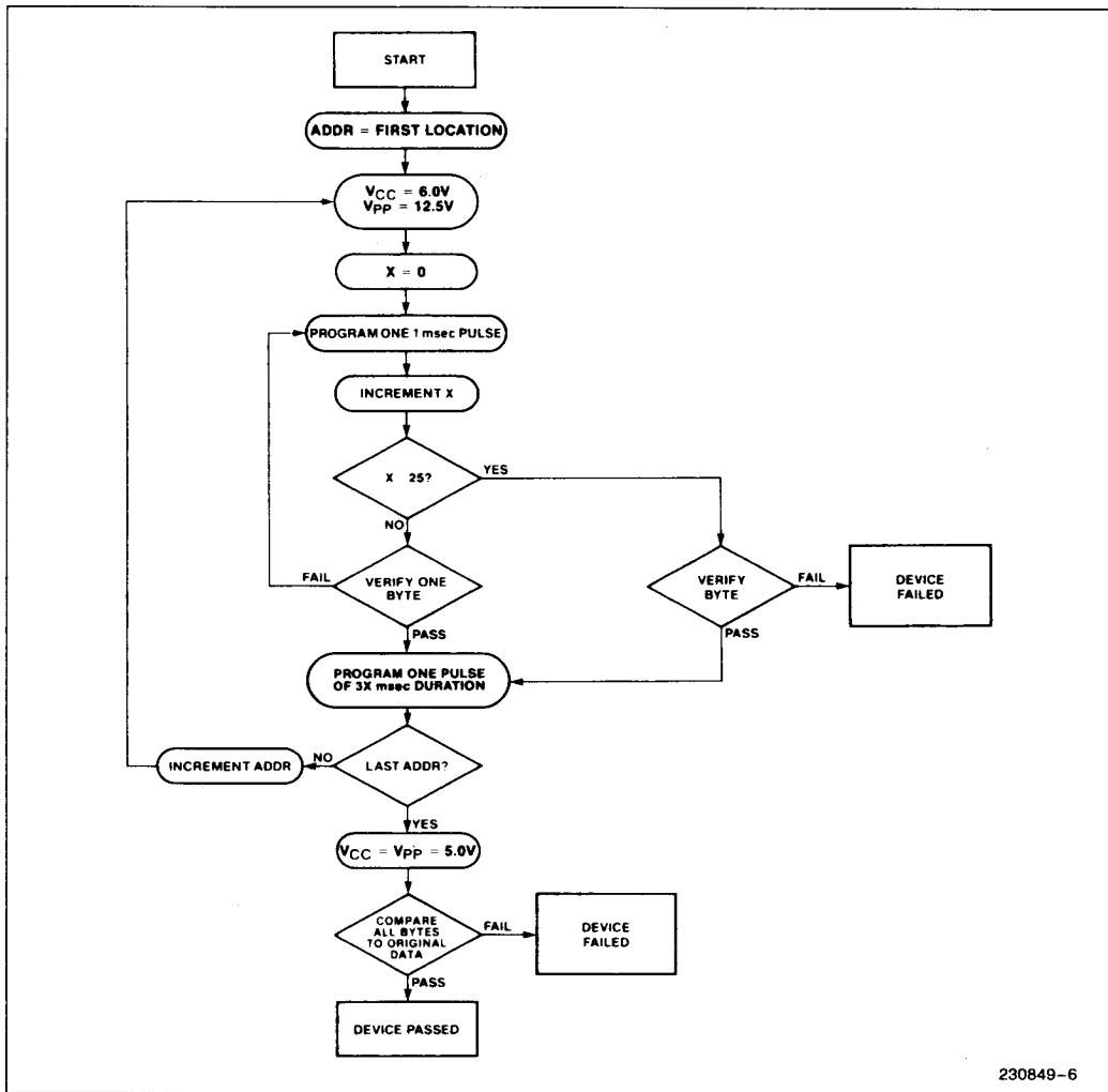
Figure 3. intelligent Programming Flowchart
