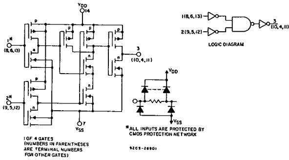
Fig. 5 - Schematic and logic diagrams for CD4001B.
