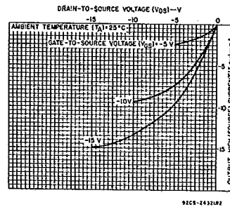
Fig. 9 - Minimum output high (source) current characteristics.
