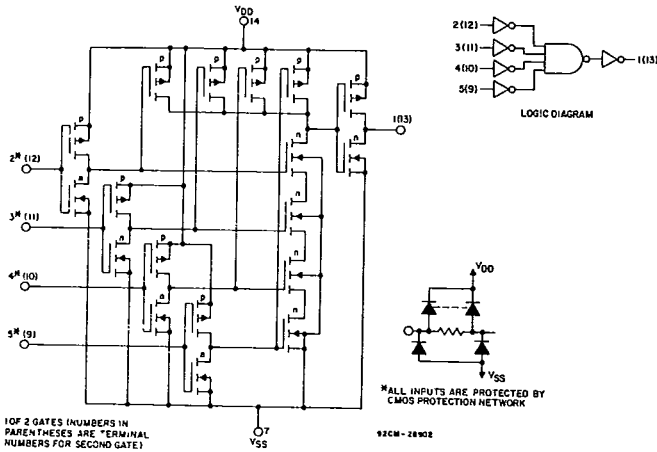
Fig. 6 - Schematic and logic diagrams for CD4002B.
