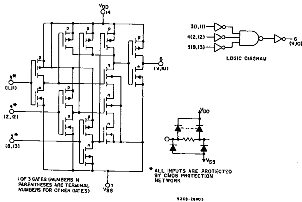
Fig. 7 - Schematic and logic diagrams for CD4025B.
