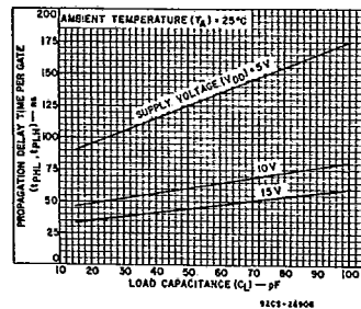
Fig. 11 - Typical propagation delay time vs. load capacitance.
