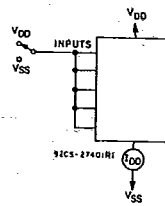
Fig. 15 - Quiescent-device current test circuit.
