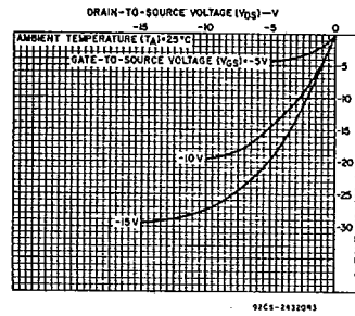
Fig. 8 - Typical output high (source) current characteristics.
