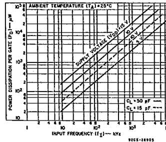
Fig. 2 - Typical power dissipation vs. frequency.
