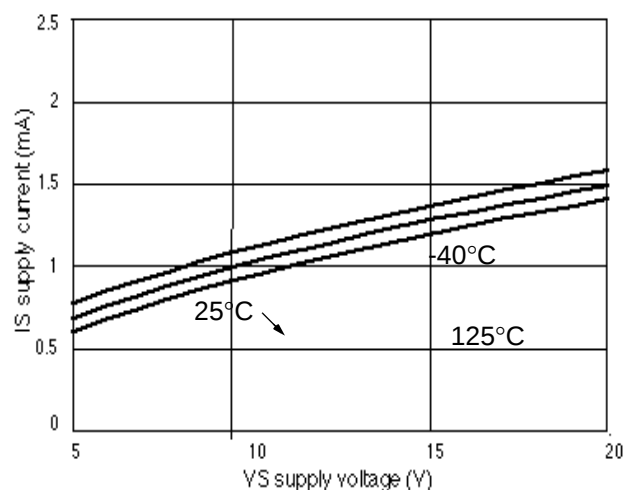
Figure 10. VS voltage versus IS current (V cc =5.5V, V dia,L , I L =20V)
