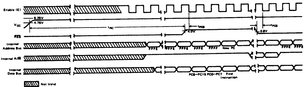
Figure 8 Reset Timing
