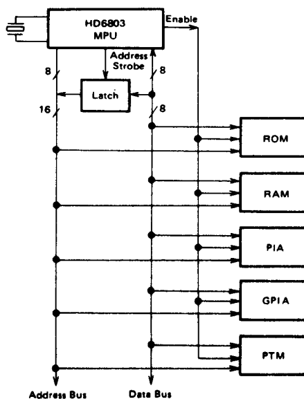
Figure 17 HD6803 MPU Expanded Multiplexed Bus
