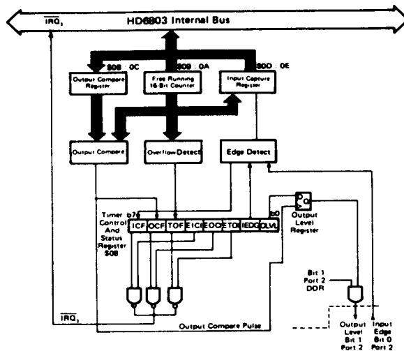
Figure 13 Block Diagram of Programmable Timer
