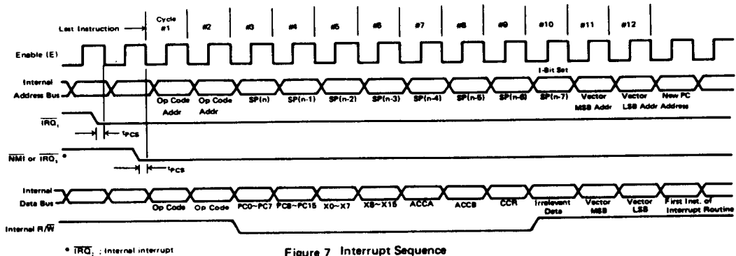
Figure 7 Interrupt Sequence
