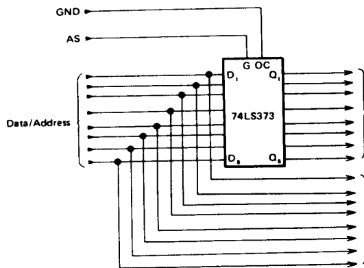
Figure 11 Latch Connection
