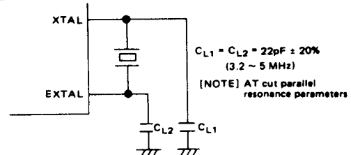
Figure 9 Crystal Interface
