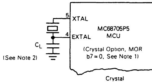
FIGURE 10 — CLOCK GENERATOR OPTIONS
