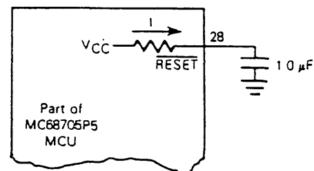
FIGURE 8 — POWER-UP RESET DELAY CIRCUIT
