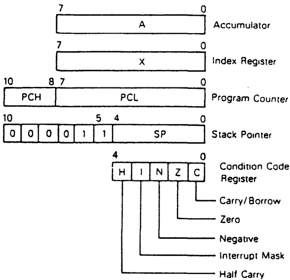
FIGURE 6 — PROGRAMMING MODEL
