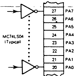
TTL Driving Port A Directly
