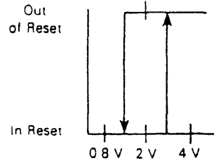
FIGURE 9 — TYPICAL RESET SCHMITT TRIGGER HYSTERESIS
