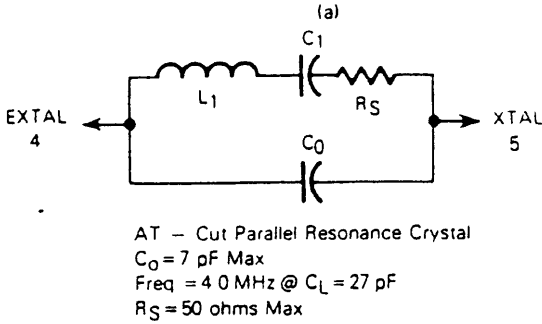
FIGURE 11 — CRYSTAL MOTIONAL-ARM PARAMETERS AND SUGGESTED PC BOARD LAYOUT
