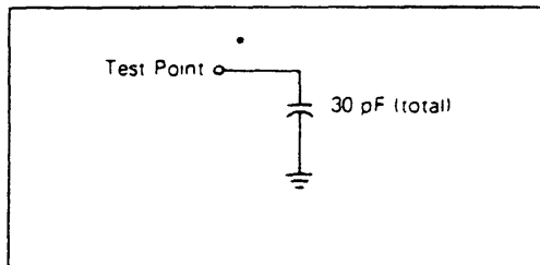
FIGURE 2 — CMOS EQUIVALENT TEST LOAD (PORT A)
