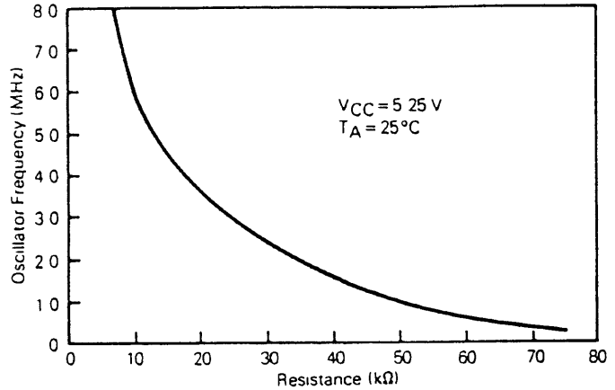
FIGURE 12 — TYPICAL FREQUENCY SELECTION FOR RESISTOR OSCILLATOR OPTION
