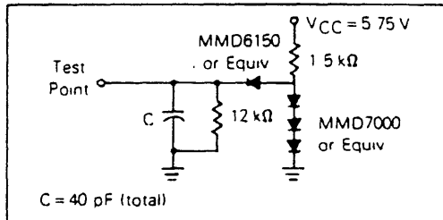
FIGURE 2 — CMOS EQUIVALENT TEST LOAD (PORT A)
