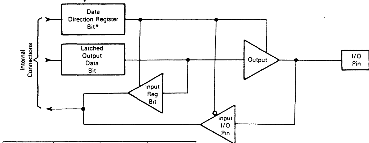
FIGURE 15 — TYPICAL PORT I/O CIRCUITRY
