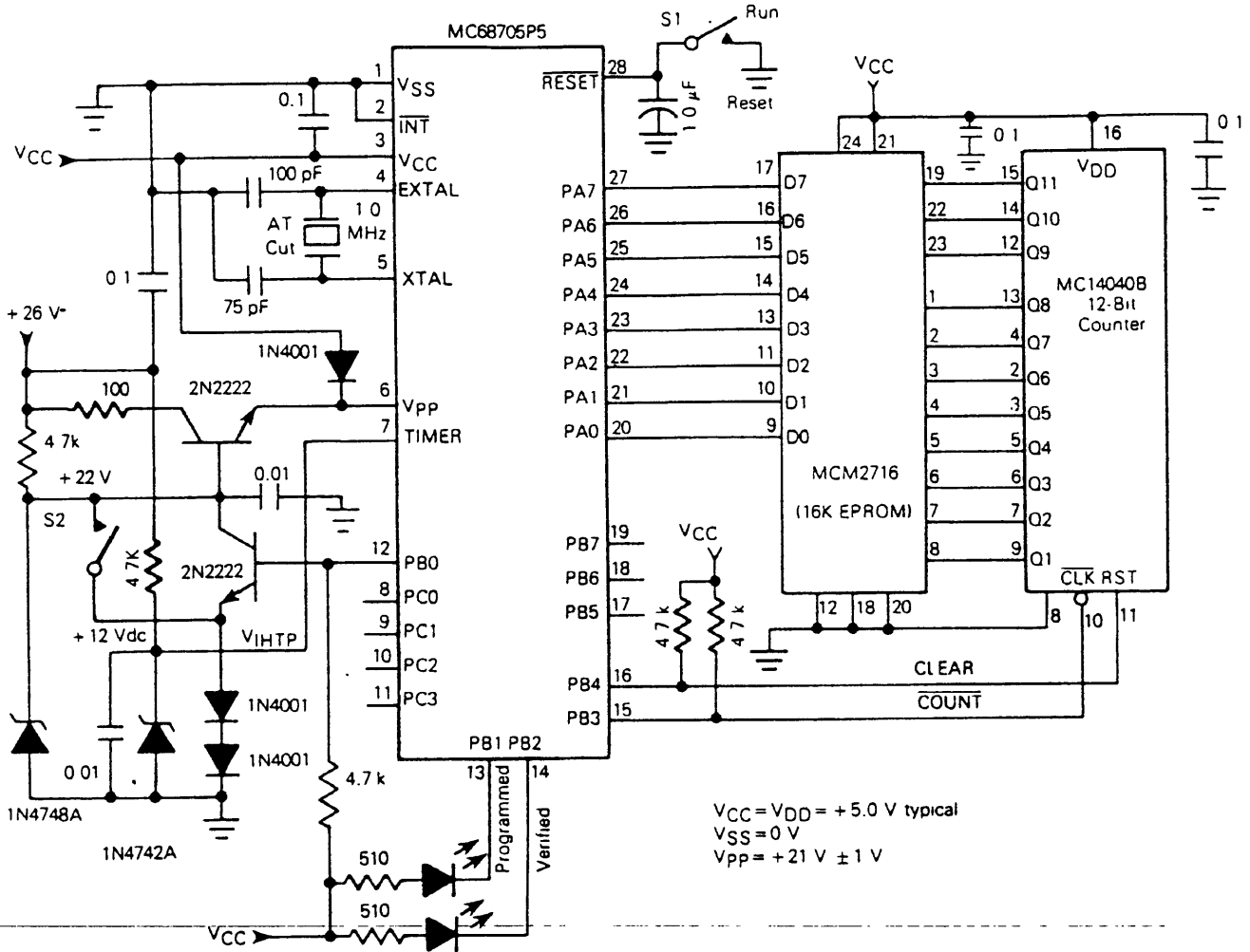
FIGURE 18 — PROGRAMMING CONNECTIONS SCHEMATIC DIAGRAM
