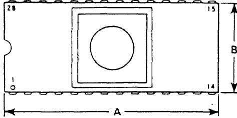
L SUFFIX CERAMIC PACKAGE CASE 719
