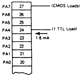
Port A, Bit 7 Programmed as Output, Driving CMOS Loads and Bit 4 Driving one TTL Load Directly (using CMOS output option)
