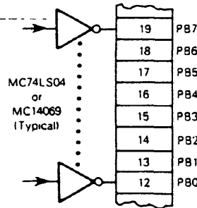
CMOS or TTL Driving Port B Directly
