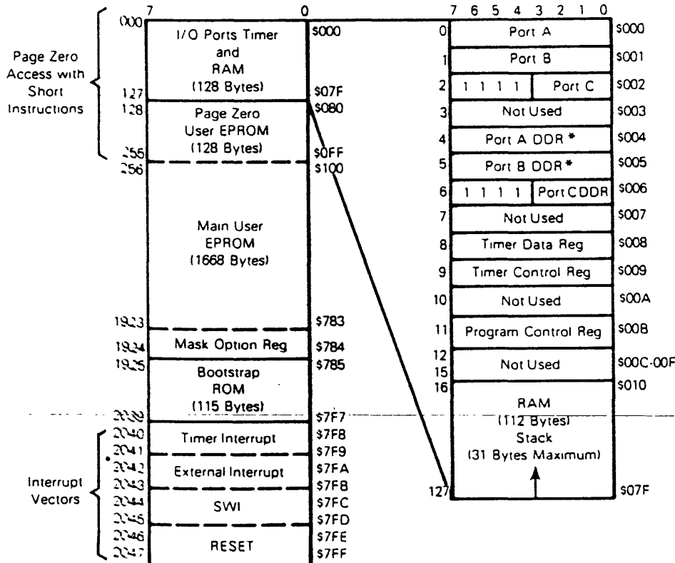
FIGURE 4 – MC68705P5 MCU MEMORY CONFIGURATION
