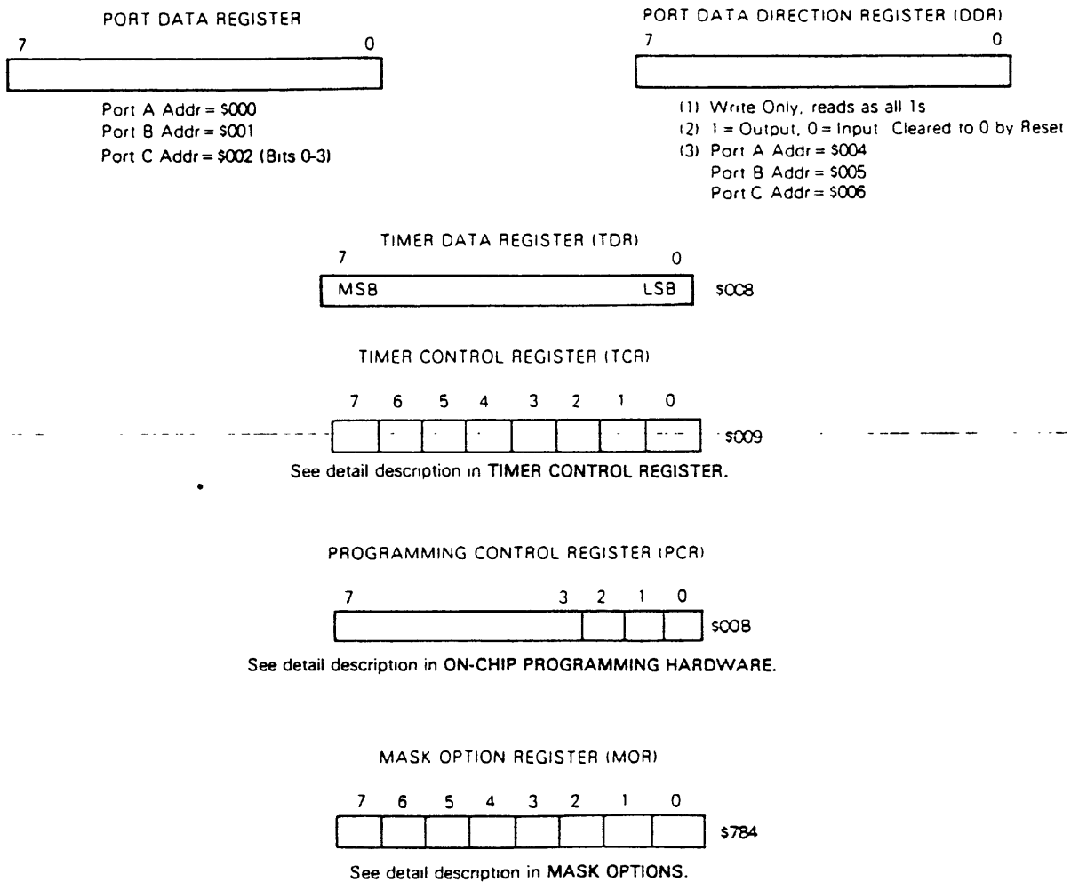
FIGURE 16 — MCU REGISTER CONFIGURATION
