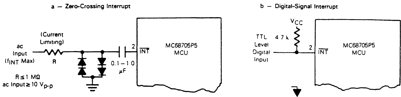
FIGURE 14 — TYPICAL INTERRUPT CIRCUITS
