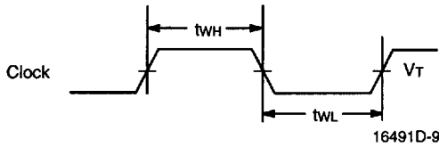
Clock Width
