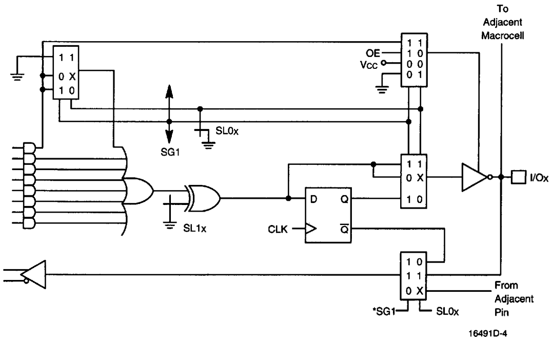
Figure 1. PALCE20V8 Macrocell
