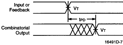
Combinatorial Output
