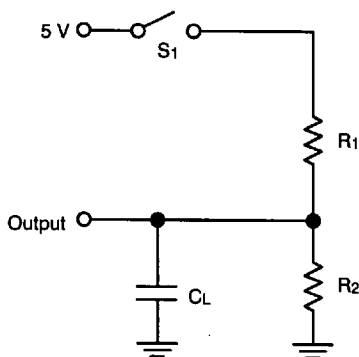
Switching Test Circuit
