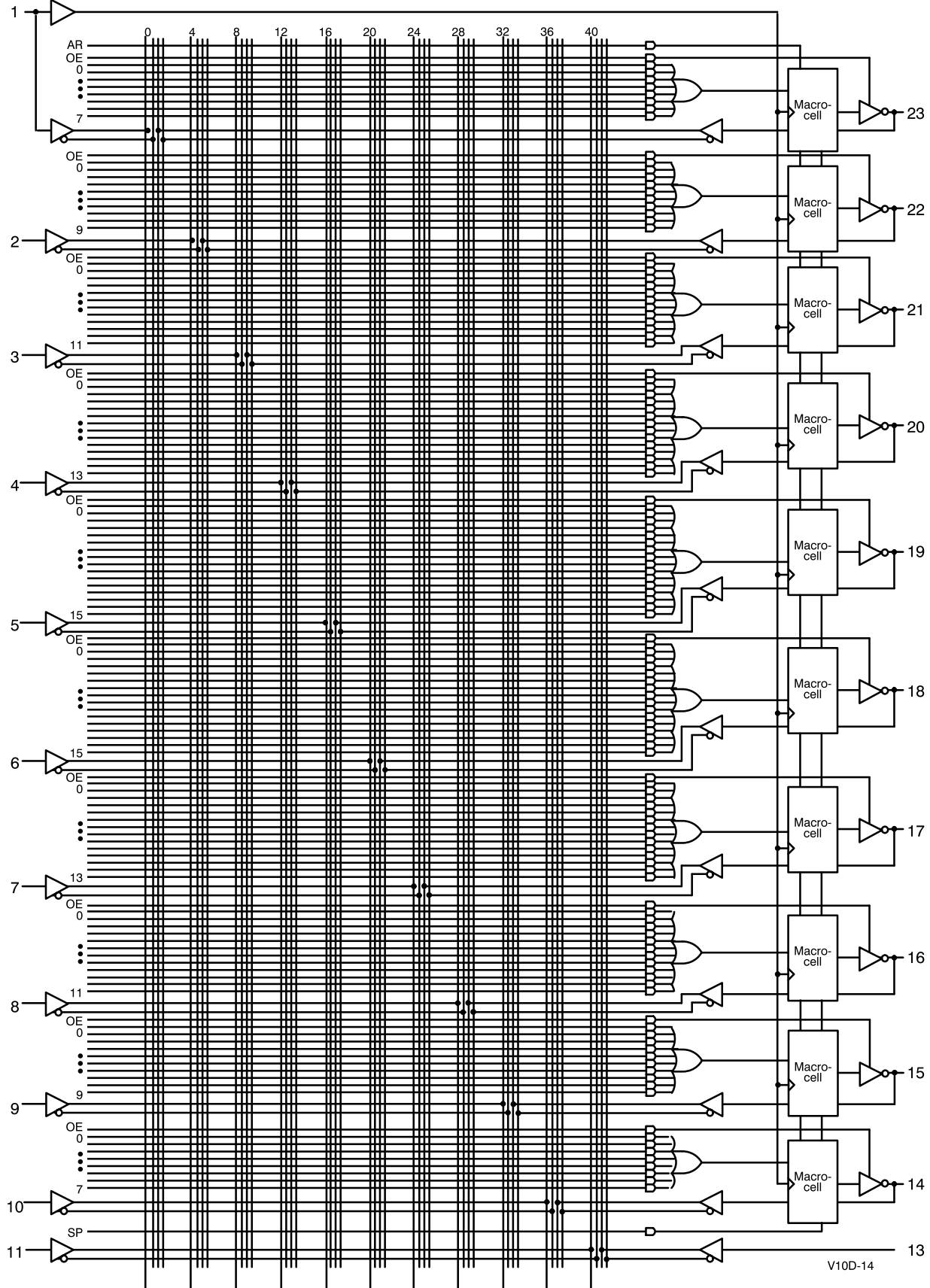
Functional Logic Diagram for PALC22V10D
