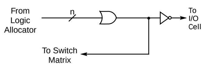
b. Combinatorial, active low
