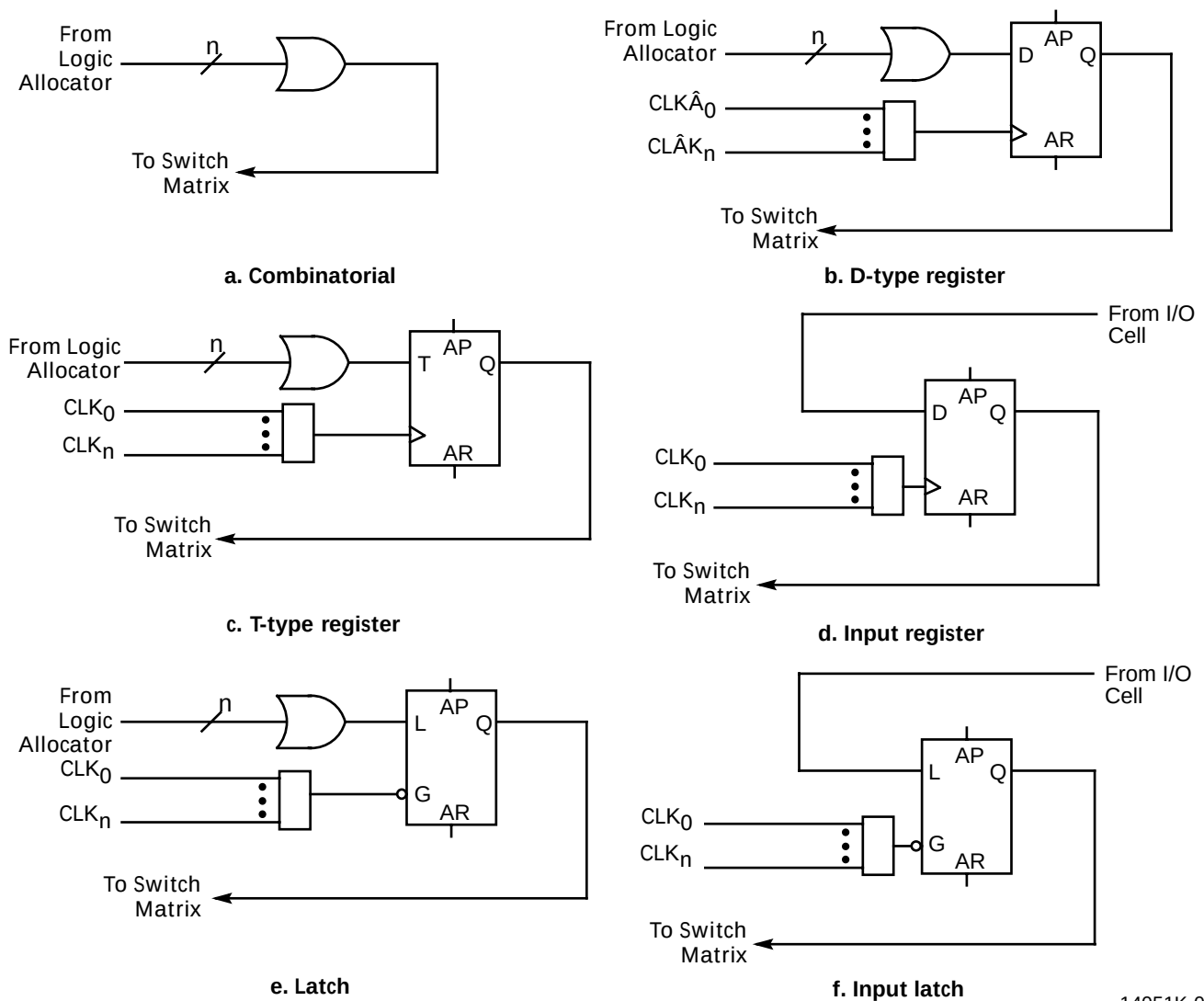
Figure 6. Buried Macrocell Configurations (MACH 2 only)
