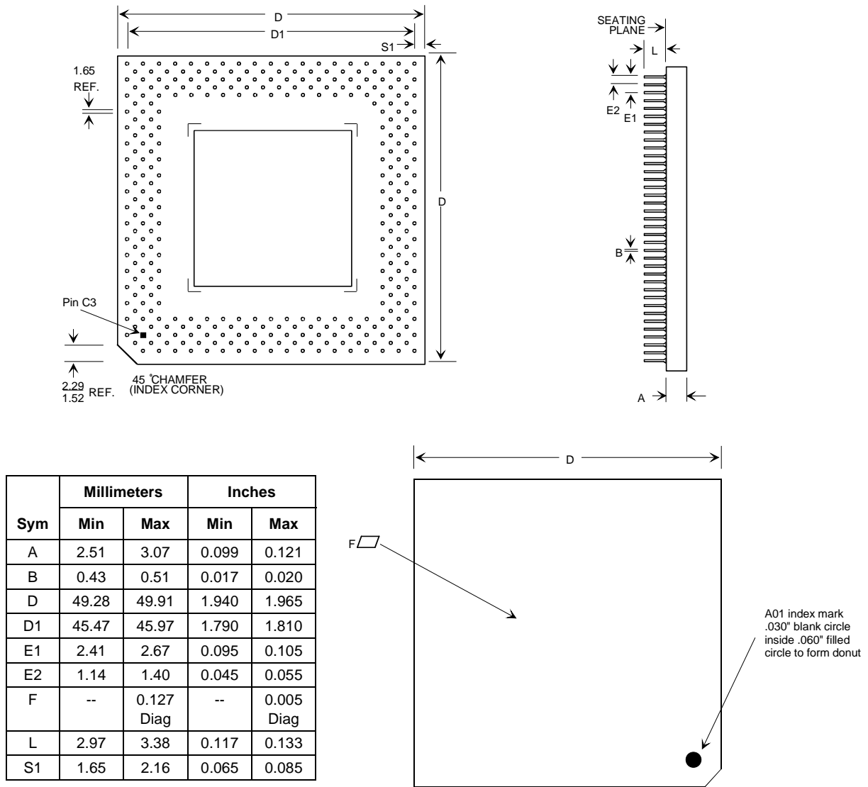
Figure 8-3. 320-Pin SPGA Mechanical Package Outline
