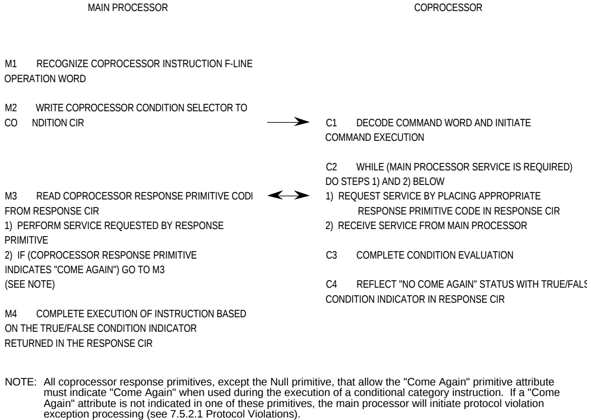
Figure 7-8. Coprocessor Interface Protocol for Conditional Category Instructions
