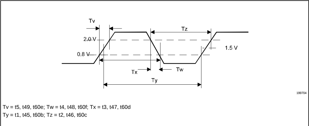
Figure 4. Clock Waveform
