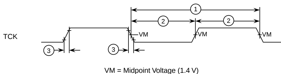
Figure 5. Clock Input Timing Diagram
