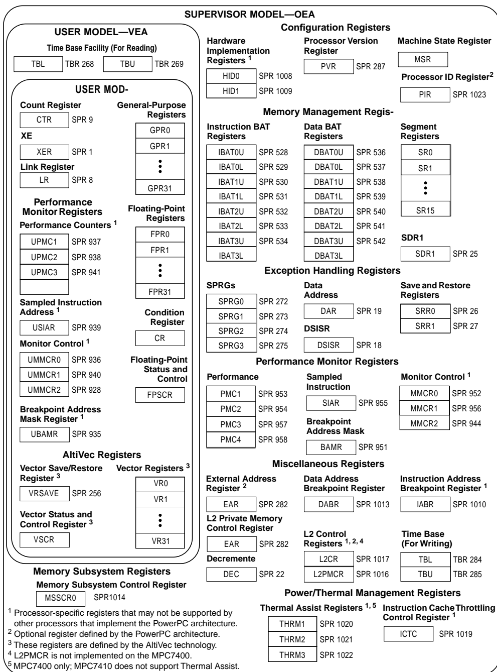
Figure 2-1. Programming Model—MPC7410 Microprocessor Registers
