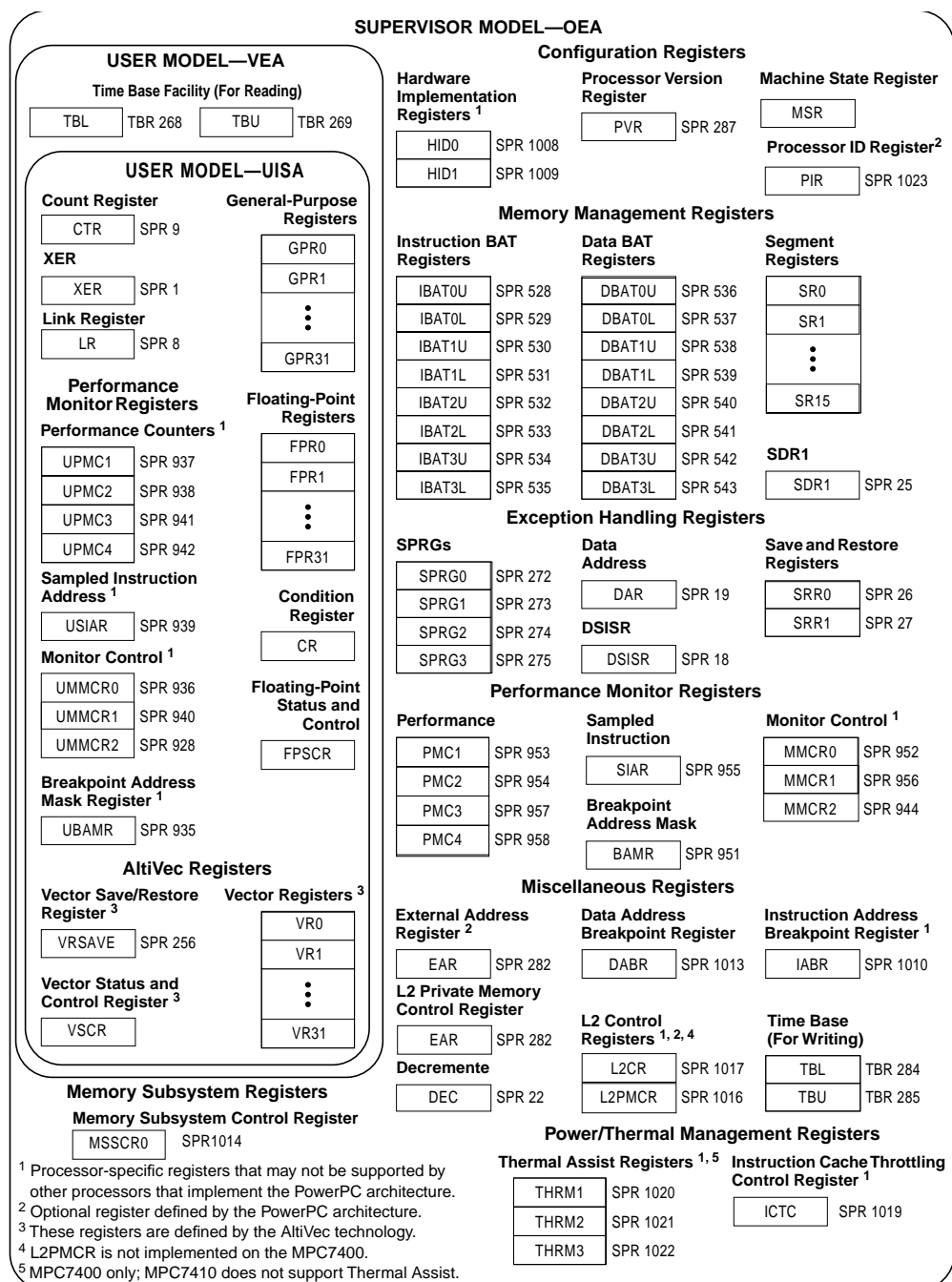
Figure 1-5. MPC7410 Microprocessor Programming Model—Registers
