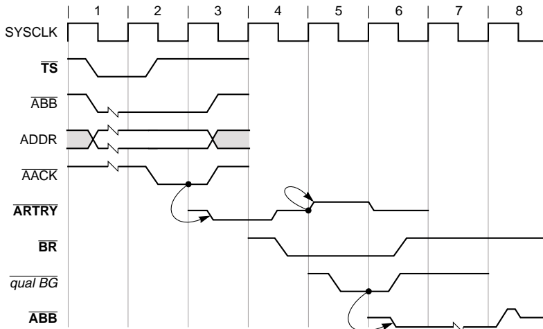
Figure 9-7. Snooped Address Cycle with \overline{\text{ARTRY}}
