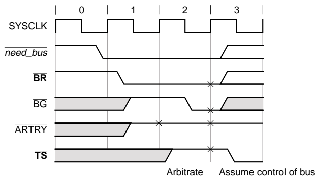
Figure 9-18. MPX Bus Address Bus Arbitration—Non-Parked Case
