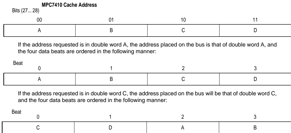
Figure 3-39. Double-Word Address Ordering—Critical Double Word First
