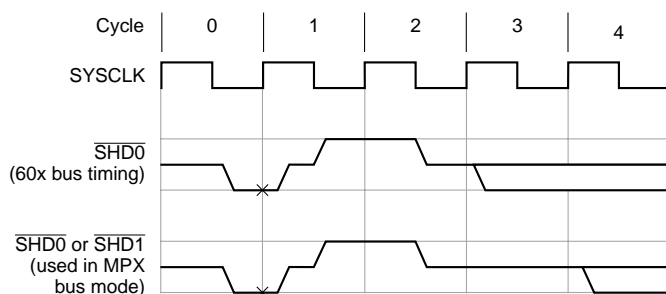
Figure 9-22. \overline{\text{SHD0}} and \overline{\text{SHD1}} Negation Timing
