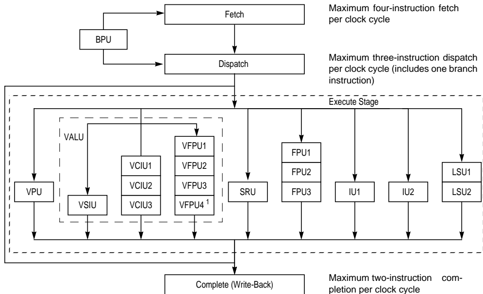
Figure 6-2. Superscalar/Pipeline Diagram
