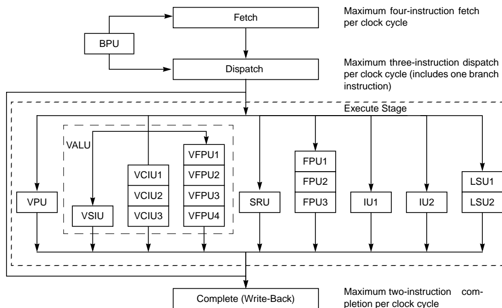
Figure 1-6. Pipeline Diagram
