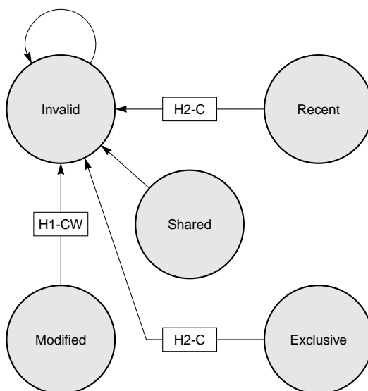
Figure 3-20. RWITM Transaction —MPX Bus Mode, L1_INTVEN = 0b111
