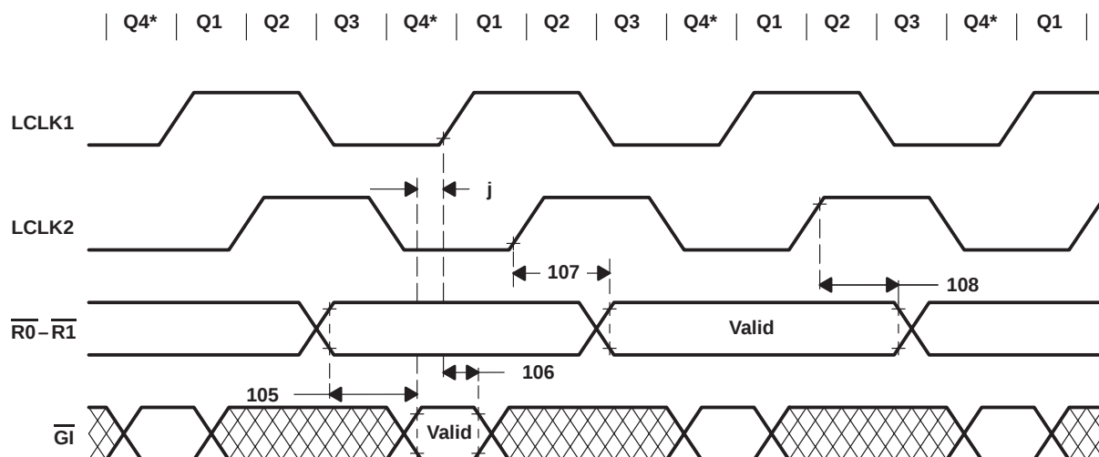
Figure 44. Multiprocessor Interface Timing: \overline{\text{GI}} , \overline{\text{ALTCH}} , \overline{\text{RAS}} , \overline{\text{R0}} and \overline{\text{R1}}
