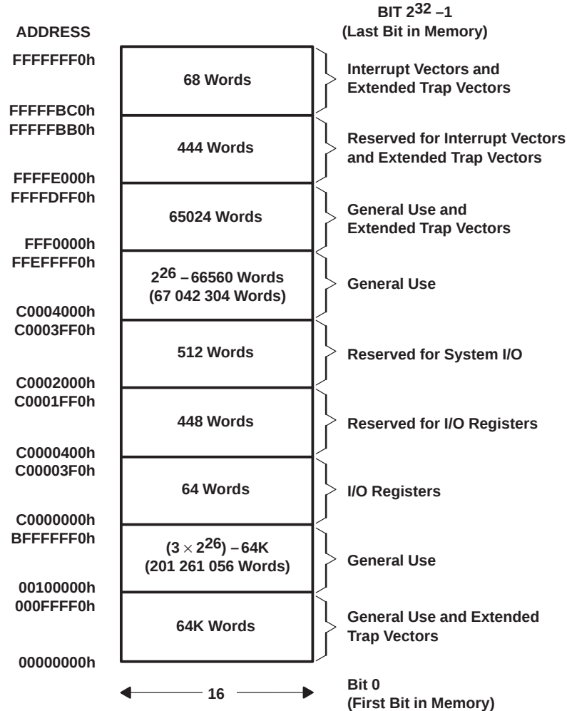
Figure 1. Memory Map
