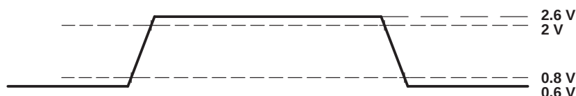
Figure 31. TTL-Level Outputs
