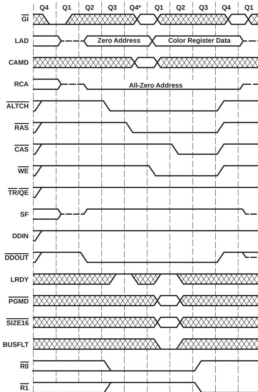
Figure 10. Load-Color-Latch Cycle
