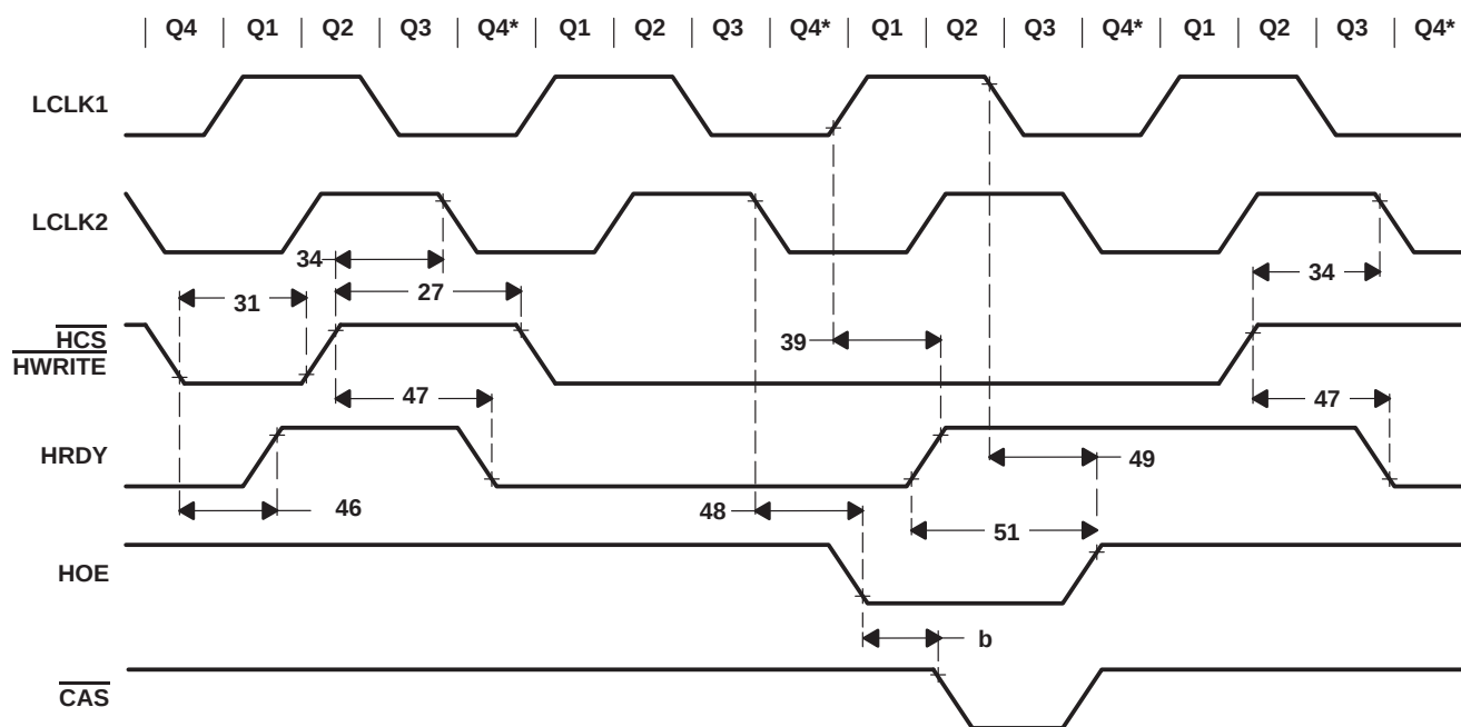
Figure 39. Host Interface Timing Responses (Write Cycle)
