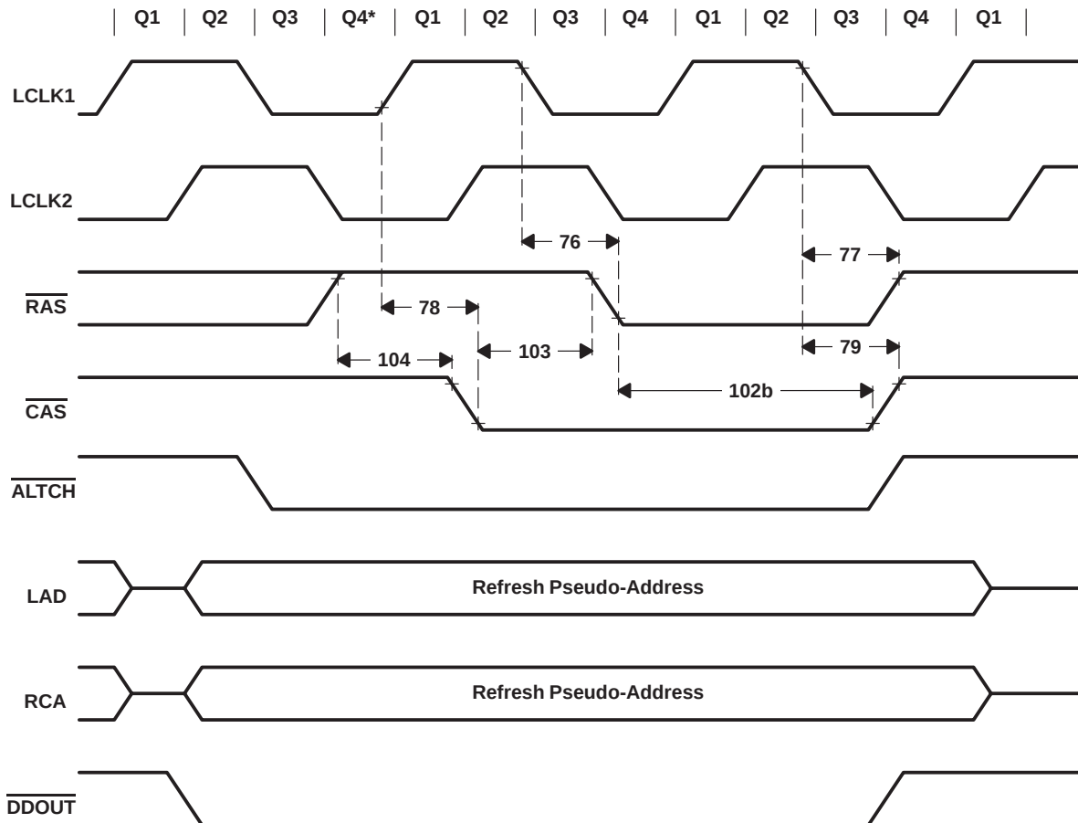
Figure 43. CAS-Before-RAS Refresh: RAS and CAS0–CAS3
