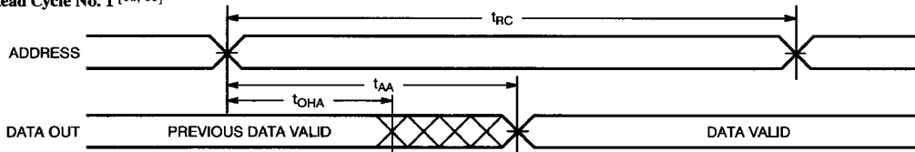
Read Cycle No. 1 [10, 11]
