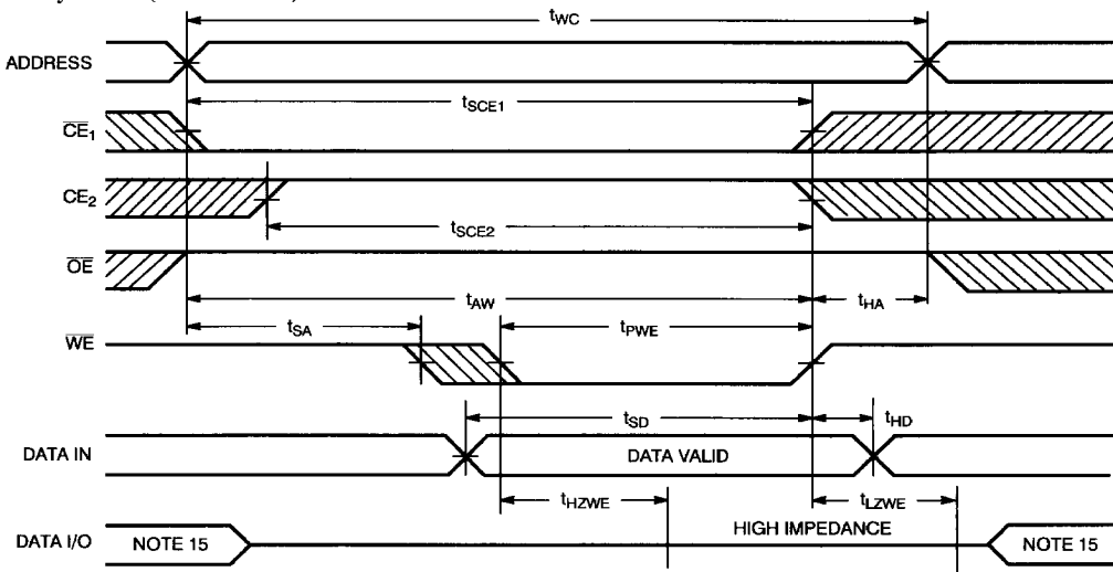
Write Cycle No. 1 ( \overline{WE} Controlled) [8, 13, 14]
