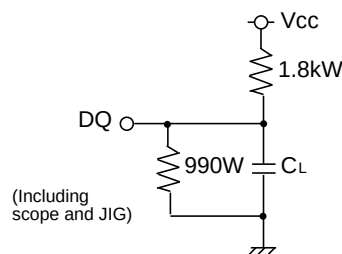
Fig.1 Output load
